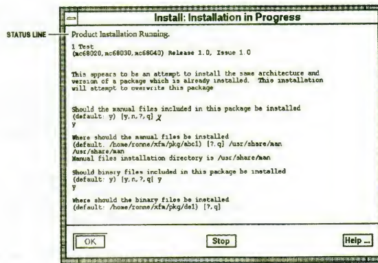
Figure 3-2 Progress Window
